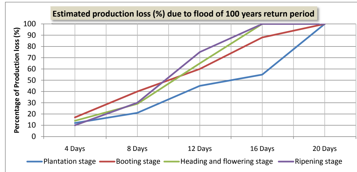
Figure 3.16 Estimated Production Loss (%) Due to Floods of 100-year Return Periods
